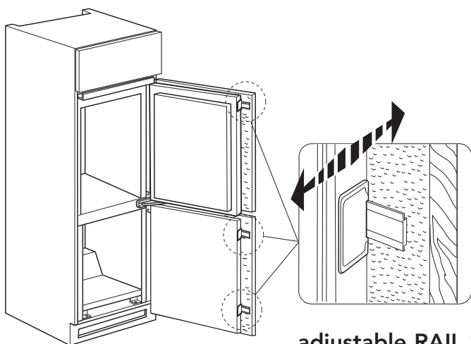
adjustable RAIL SYSTEM with cover screws
