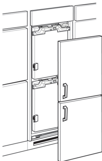
adjustable RAIL SYSTEM with cover screws
