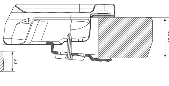
Plan 30-60 mm
