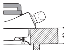
Hooking position for top H=40mm
